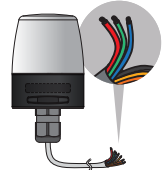
The Red, Green and Blue wires achieve 7 colors
